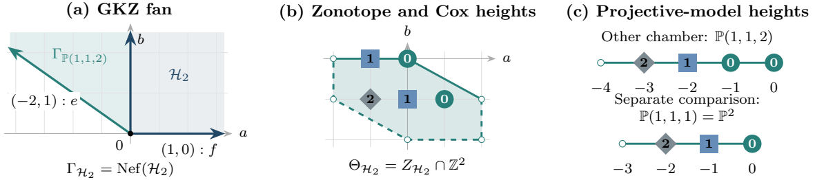
FIGURE 3. Birational models and diagonal heights for \mathcal{H}_2 . (a) GKZ chambers; contracting the (-2) -section e gives the coarse space of \mathbb{P}(1, 1, 2) . (b) The common zonotope Z_{\mathcal{H}_2} = Z_S , with Cox-category heights from the minimal uniform diagonal. (c) Heights on the projective models, with \mathbb{P}^2 shown as a separate comparison [47, §4].
