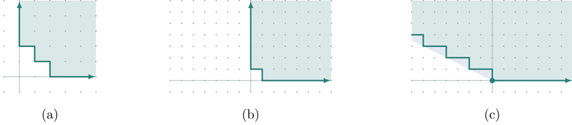
FIGURE 1. Regularity regions of (a) S/I_Z for three points Z = \{([1:1], [1:4]), ([1:2], [1:5]), ([1:3], [1:6])\} \subset \mathbb{P}^1 \times \mathbb{P}^1 ; (b) \mathcal{O}_{\mathcal{H}_2} ; (c) S/I_p for a point p \in \mathcal{H}_2 .
